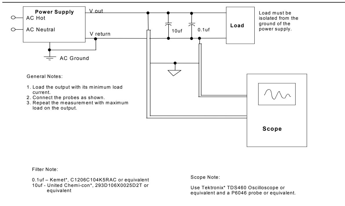
Figure 4. Differential Noise Test Setup
